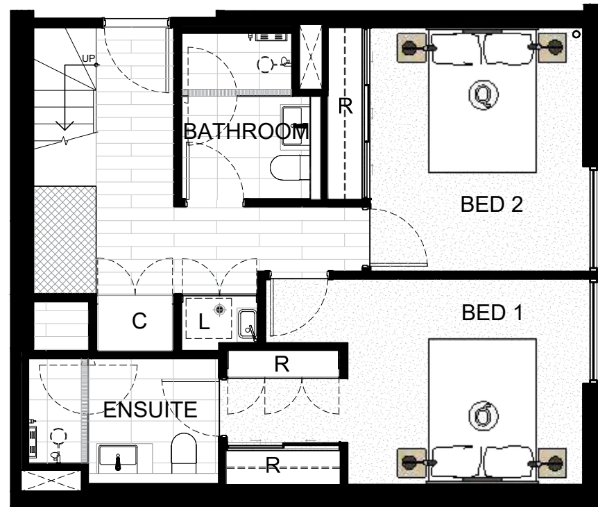
LEVEL 1 PLAN
