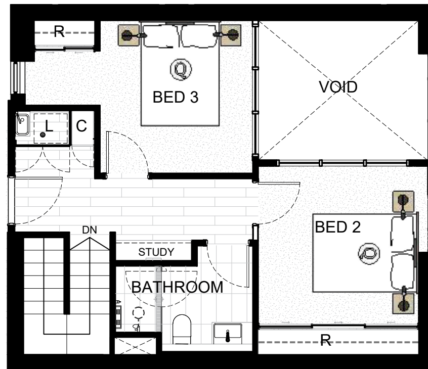
LEVEL 2 PLAN
